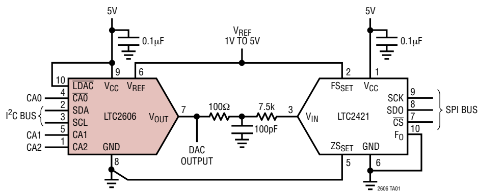
Demo Circuit Schematic. Onboard 20-Bit ADC Measures Key Performance Parameters
