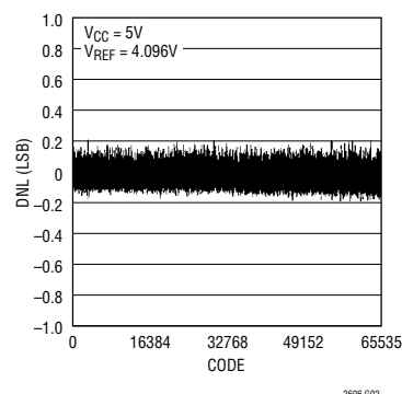
Differential Nonlinearity (LTC2606)
